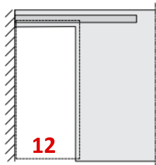
Single Sliding Door Next to a Wall
