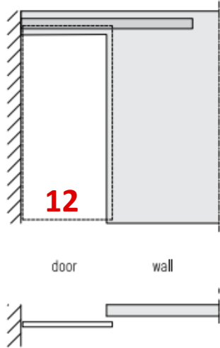
Single Sliding Door Next to a Wall
